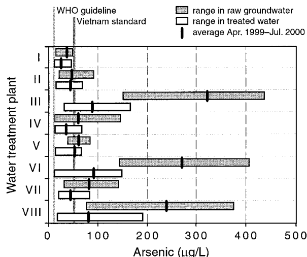
FIGURE 2. Arsenic concentration ranges in raw groundwaters from the lower aquifer and in treated Hanoi waters of eight water treatment plants. Seven sample series were analyzed from April 1999 through July 2000 ( 7 \times 16 samples). The numbers I–VIII of the water works refer to Figure 1. The full database is available as Supporting Information.
